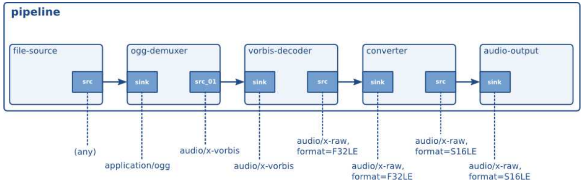
Figure 18-1. The Hello world pipeline with media types
