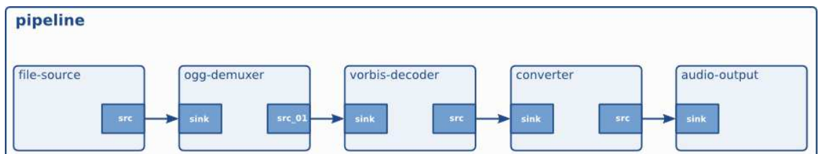
Figure 10-1. The "hello world" pipeline
