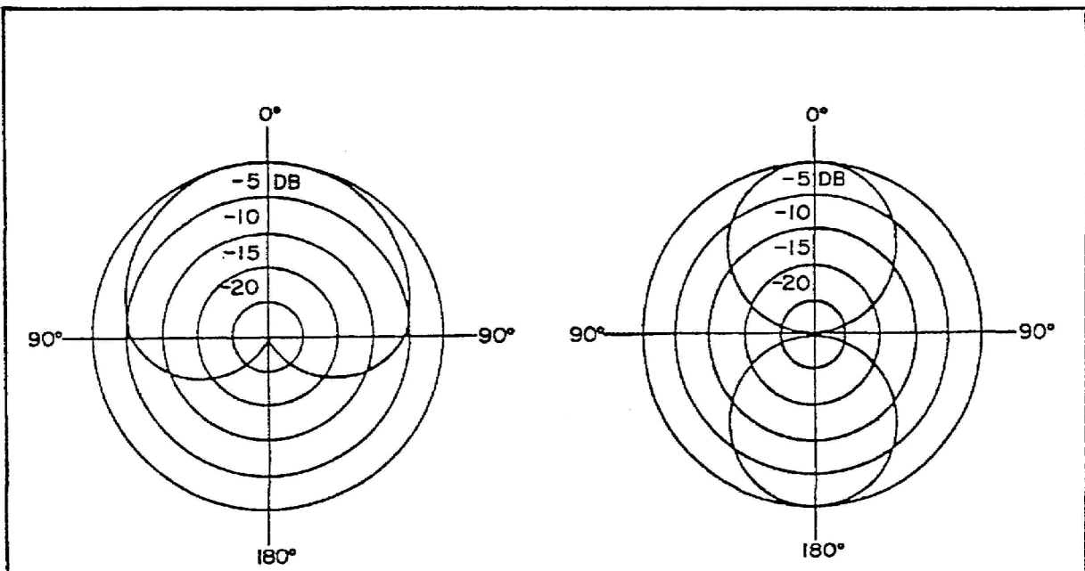
Figure 2-3 Unidirectional
