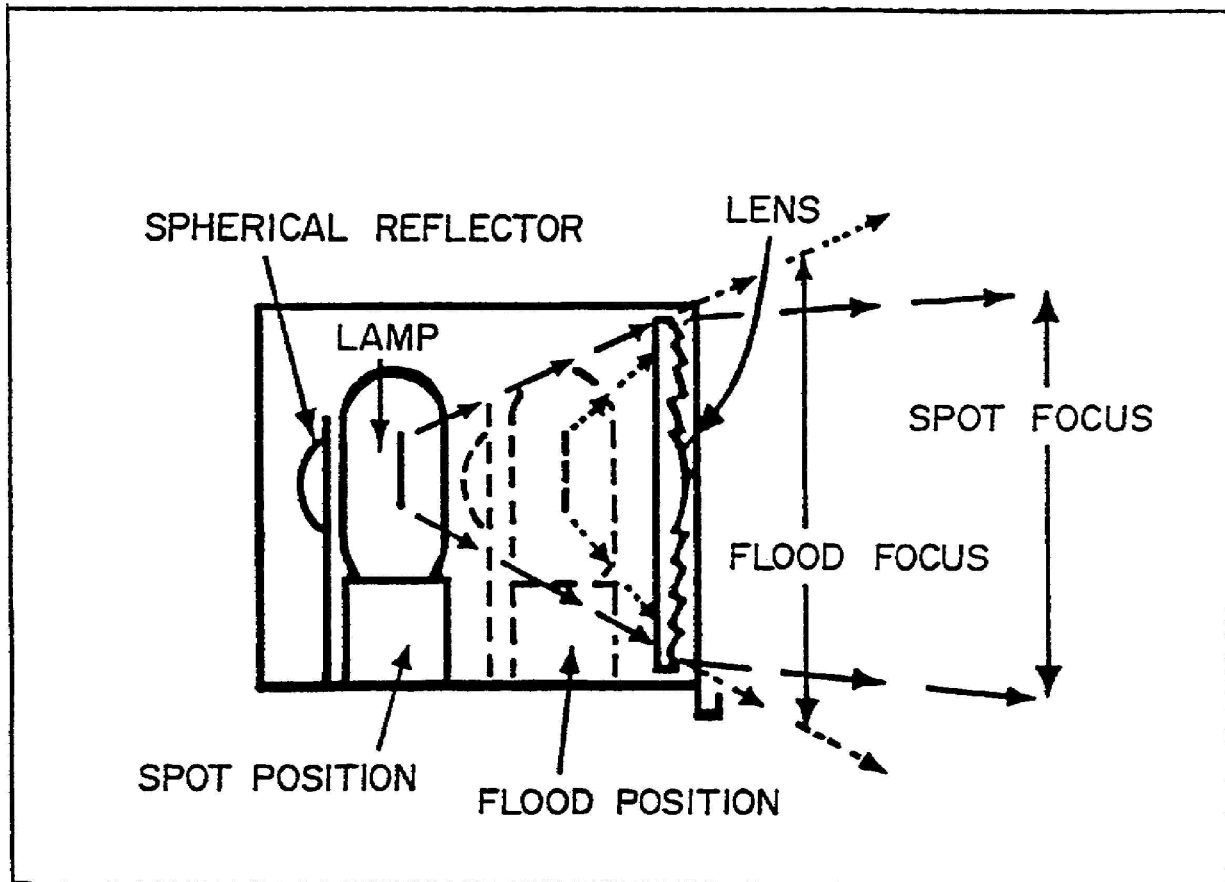
Figure 1-4 Spotlight
