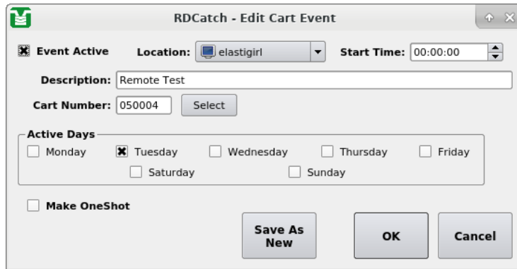
The Edit Cart Event Dialog
